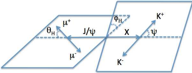
FIG. 11: Definition of the decay angles \theta_H , \phi_H , and \psi in the helicity basis for the sequential decay B_s^0 \rightarrow J/\psi f_2'(1525) , J/\psi \rightarrow \mu^+ \mu^- , X \rightarrow K^+ K^- .
