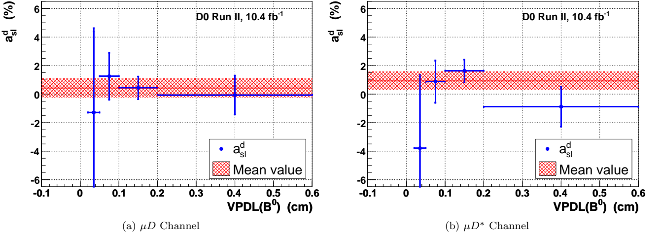
FIG. 7: Final measurements of the semileptonic asymmetry a_{sl}^d , in bins of VPDL( B^0 ), for both channels. The cross-hatched bands show the mean values (and their total uncertainties) determined for each channel separately.
