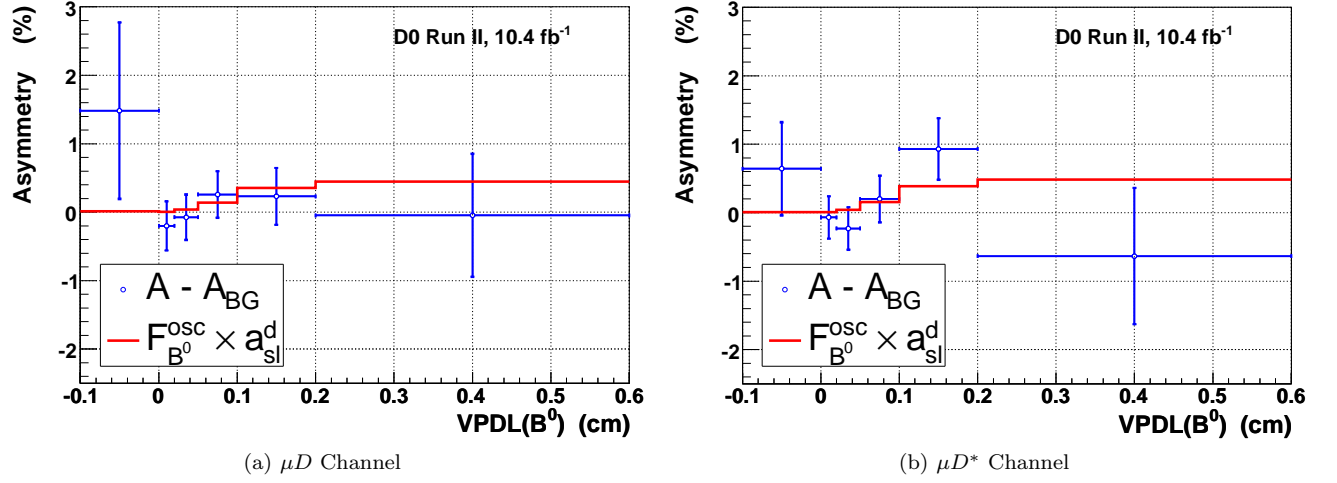
FIG. 8: Final measurements of the background corrected asymmetry, in bins of \text{VPDL}(B^0) , for both channels. The points show the observed asymmetry, with the solid lines showing F_{B^0}^{\text{osc}} \cdot a_{\text{sl}}^d . Any asymmetry caused by mixing should exhibit a characteristic turn-on shape as the fraction of oscillated B^0 mesons increases.
