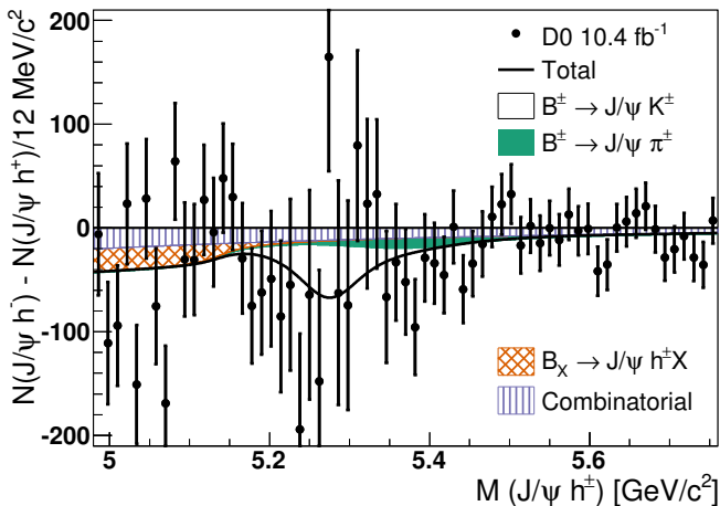
FIG. 2. The fit to the difference distribution for the data optimized for A_{\text{raw}}^{J/\psi K^\pm} (the fit is described in the text).
