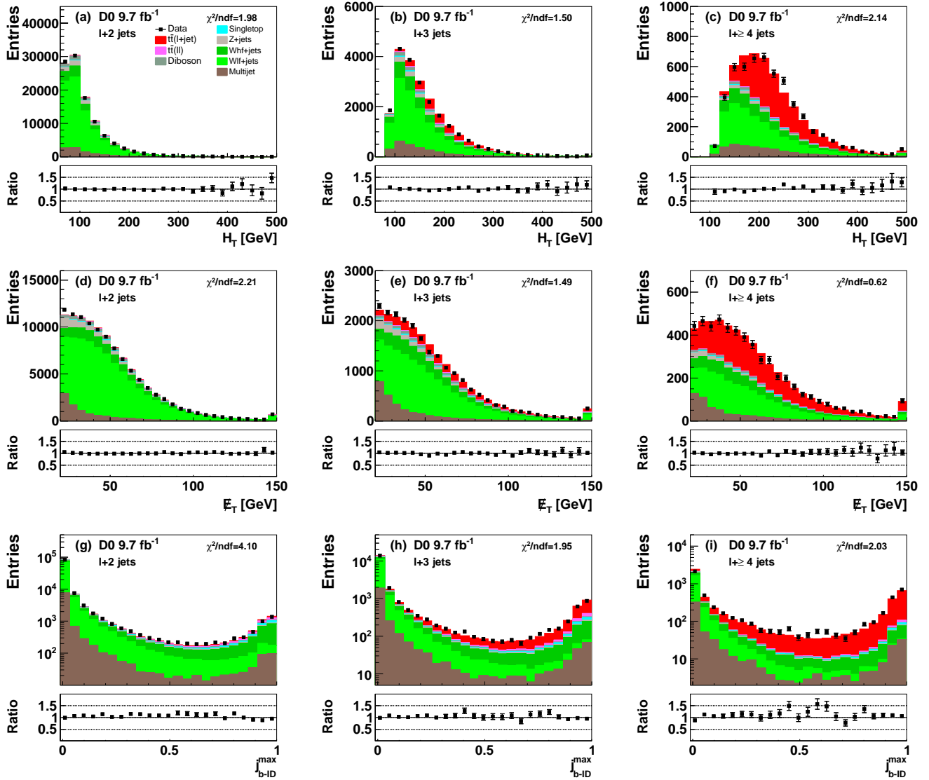
FIG. 1. Distributions of (a)–(c) the scalar sum of the p_T values of the lepton and jets, H_T , (d)–(f) \cancel{E}_T and (g)–(i) the maximal MVA b -ID value of all jets, j_{b-ID}^{\max} , for events with a lepton and two, three or four or more jets. The data are compared to the sum of predicted contributions from signal and background processes, using the theoretical value of the inclusive t\bar{t} cross section of 7.48 pb [37] and m_t = 172.5 GeV. The highest bin in the histograms includes overflows. The ratios of data to the sum of the signal and all background contributions are shown in the panels below the individual distributions. Only statistical uncertainties of the data are shown and the \chi^2/\text{ndf} values only take statistical uncertainties into account.
