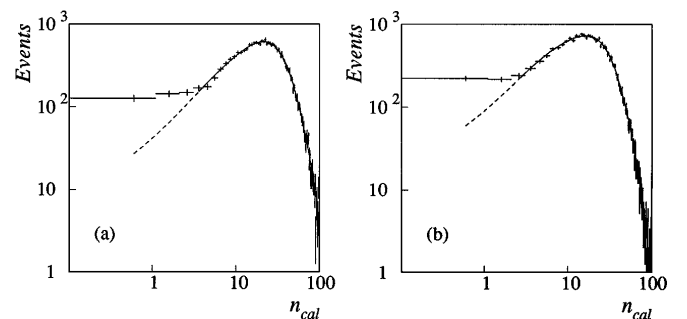
FIG. 3. The number of events vs n_{cal} (shifted up by half a unit in multiplicity) is plotted on a log-log scale for all opposite-side jet events, where (a) shows the multiplicity between the cone edges of the two leading jets and (b) shows the multiplicity in the region |\eta| < 1 . The solid lines represent the double NBD fits for (a) n_0 = 3 and (b) n_0 = 2 , while the dashed lines show the extrapolation of each fit to n_{cal} = 0 .
