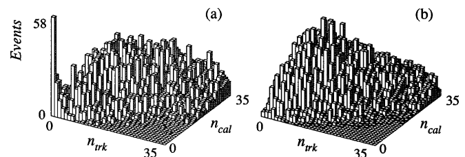
FIG. 1. The calorimeter tower multiplicity ( n_{cal} ) vs the charged track multiplicity ( n_{trk} ) in the pseudorapidity region |\eta| < 1.3 for the (a) opposite-side and (b) same-side samples as described in the text.
