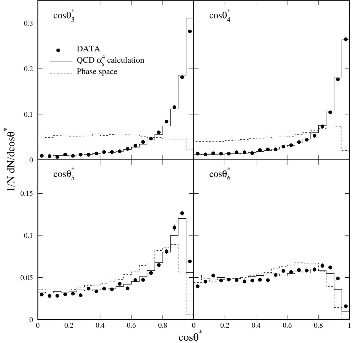
FIG. 8. The distributions of jet polar angle for the four-jet events in their center-of-mass system. Only statistical errors are shown. The RMS's of the fractional differences between the data and QCD are 6.8%, 6.2%, 7.5% and 7.9% for \cos\theta_3^* , \cos\theta_4^* , \cos\theta_5^* and \cos\theta_6^* respectively. The estimated systematic uncertainty on the measurement is 6%. The data are also listed in Table V.
