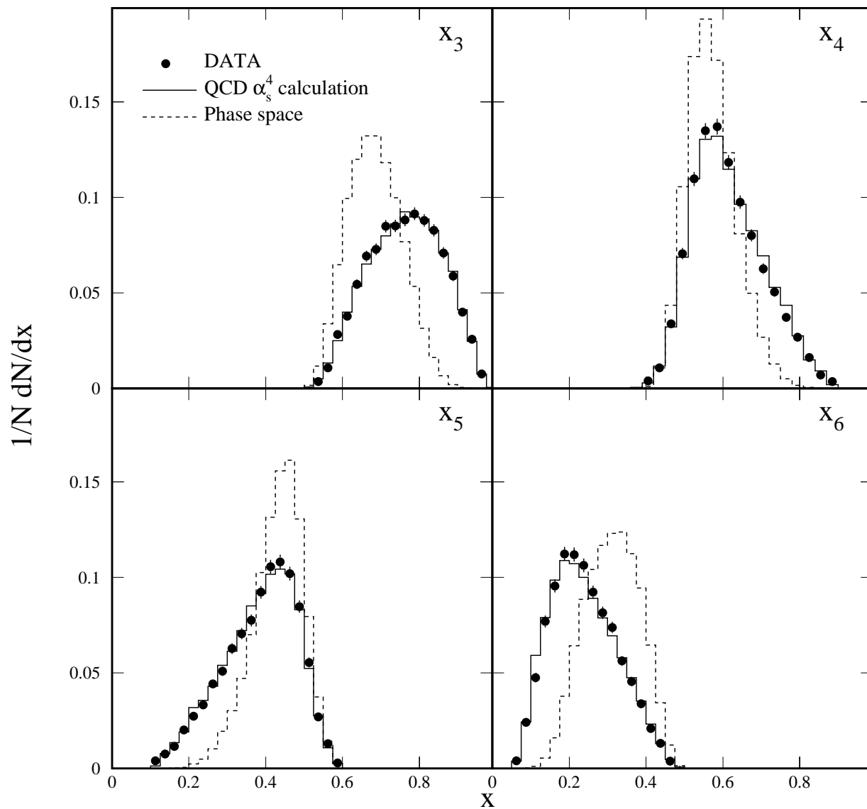
FIG. 7. The jet energy fraction distributions for the four-jet events in their center-of-mass system. Only statistical errors are shown. The RMS's of the fractional differences between the data and QCD are 6.5%, 5.5%, 6.2% and 6.5% for x_3 , x_4 , x_5 and x_6 respectively. The estimated systematic uncertainty on the measurement is 6%. The data are also listed in Table IV.
