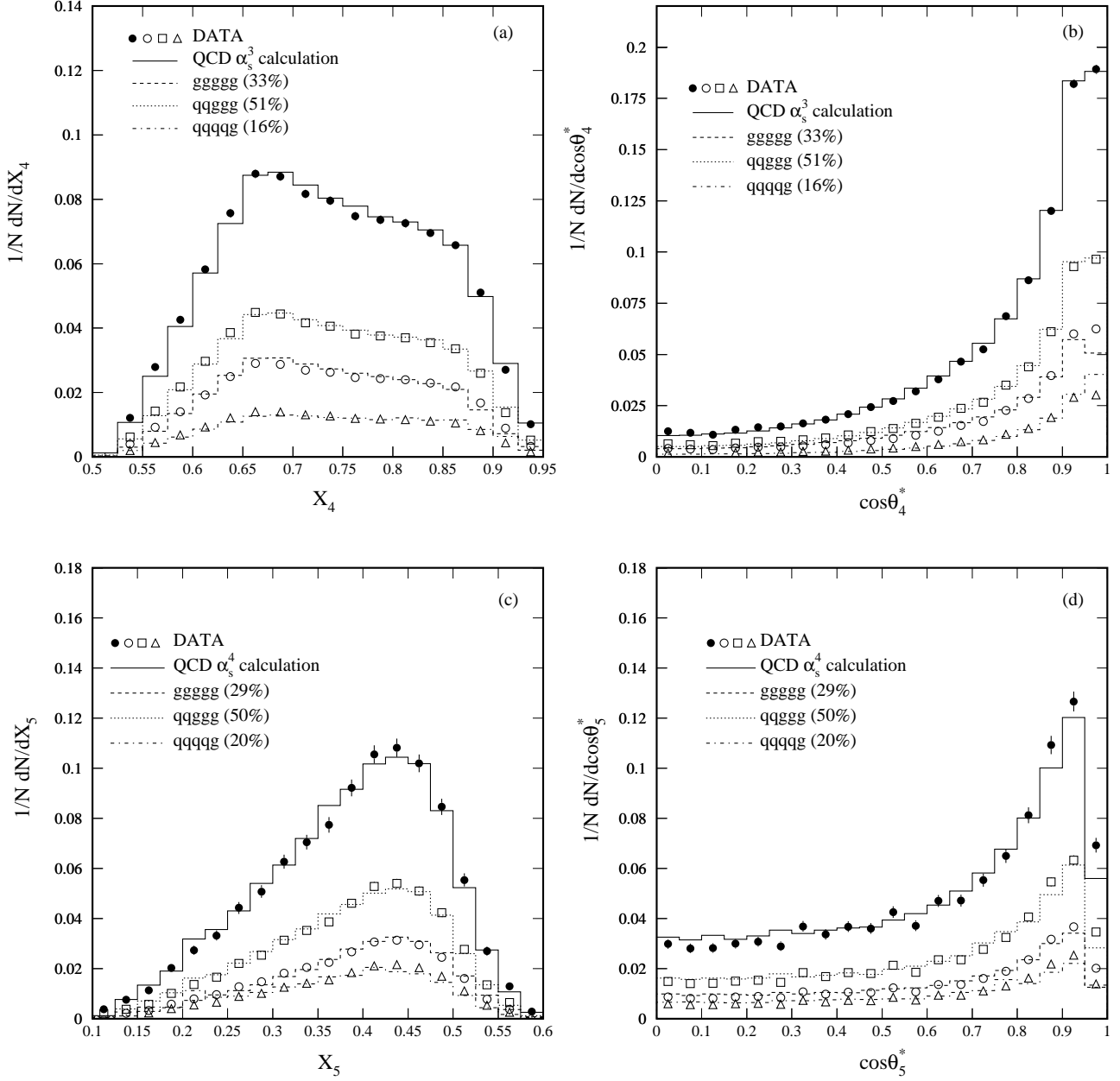
FIG. 12. The (a) x_4 and (b) \cos\theta_4^* distributions for three-jet events and the (c) x_5 and (d) \cos\theta_5^* distributions for four-jet events in their center-of-mass system. The QCD subprocesses are normalized to their fractional contributions to the respective total cross section for the selection criteria described in the text. The data are scaled to the normalization of the respective subprocess. Therefore, only the shapes of the subprocesses are compared. The estimated uncertainty on the data is less than 6%.
