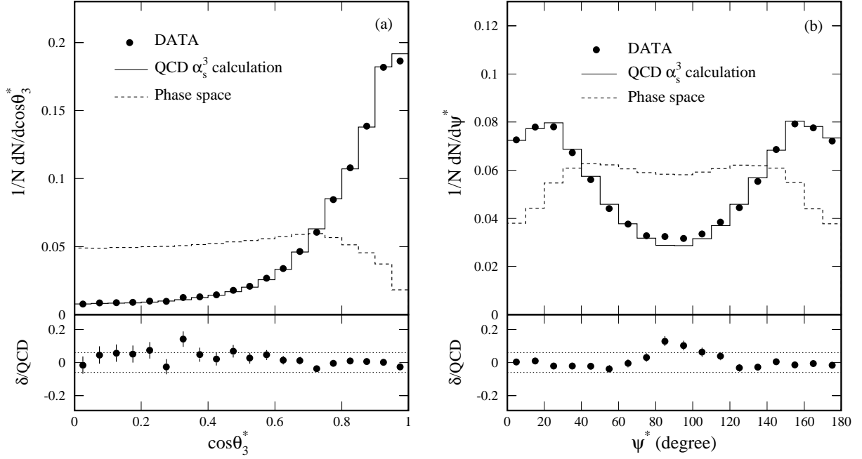
FIG. 5. The distributions for the three-jet events of (a) the cosine of the leading jet polar angle and (b) the angle \psi^* (defined in the text) in their center-of-mass system. The RMS of the fractional differences is 3.4% for \cos\theta_3^* and 4.2% for \psi^* . The dotted lines show the estimated 6% systematic uncertainty on the measurement. The data are also listed in Table II.
