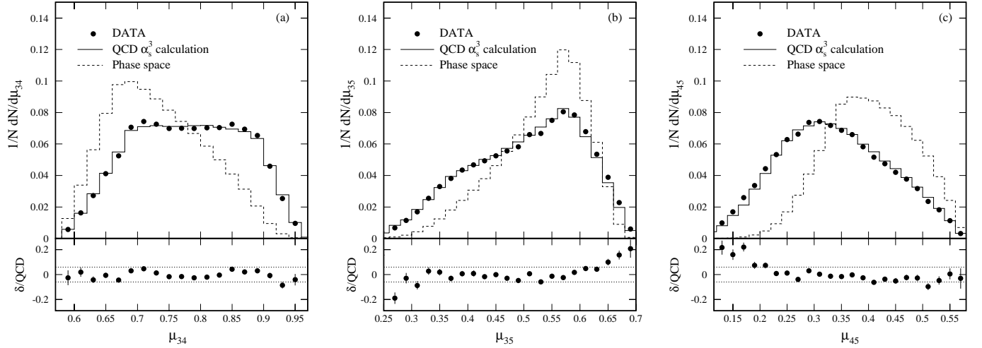
FIG. 6. The scaled mass distributions of (a) \mu_{34} , (b) \mu_{35} and (c) \mu_{45} for the three-jet events in their center-of-mass system. The bottom plots show fractional differences between the data and QCD. The RMS's of the fractional differences are 3.6%, 6.7% and 6.9% respectively. The dotted lines show the 6% systematic uncertainty on the measurement. The data are also listed in Table III.
