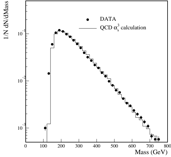
FIG. 3. The mass distributions of the selected three- and four-jet events before the mass requirement. The QCD matrix element calculations are normalized to the data.
