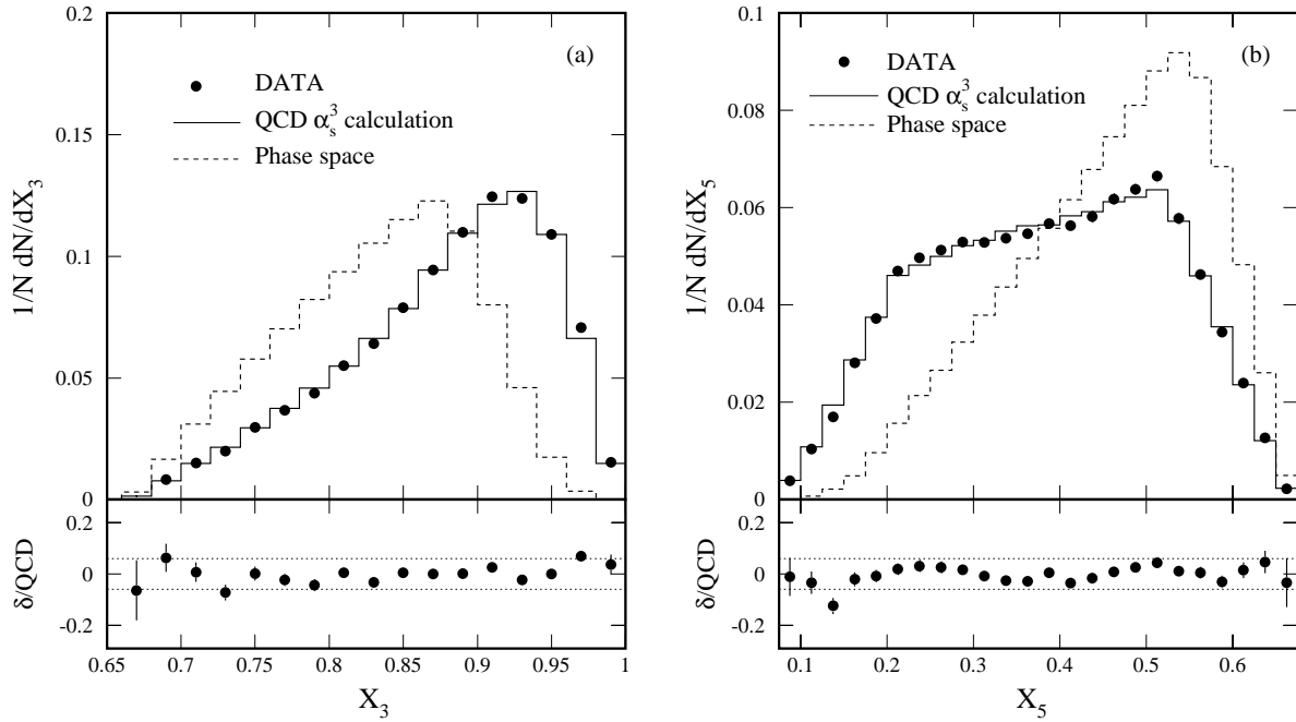
FIG. 4. The scaled energy distributions of (a) x_3 and (b) x_5 for three-jet events in their center-of-mass system. Only statistical errors are shown. The bottom plot shows the fractional difference of the data from the exact tree-level QCD calculation. The RMS of the fractional differences is 3.4% for x_3 and 3.9% for x_5 . The dotted lines show the estimated 6% systematic uncertainty on the measurement. The data are also listed in Table I.
