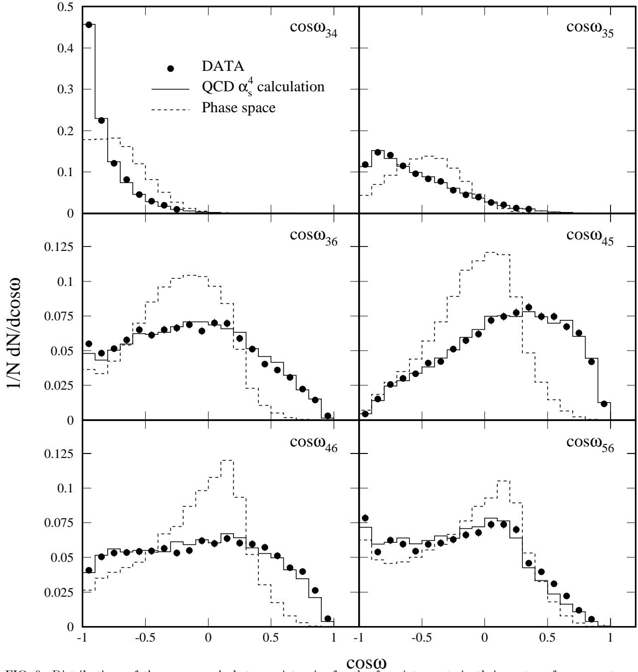
FIG. 9. Distributions of the space angle between jet pairs for the four-jet events in their center-of-mass system. Only statistical errors are shown. The RMS's of the fractional differences between the data and QCD for the six space angles are 5.4%, 5.6%, 6.4%, 4.7%, 7.6% and 8.0%. The estimated systematic uncertainty on the measurement is 6%. The data are also listed in Table VI.
