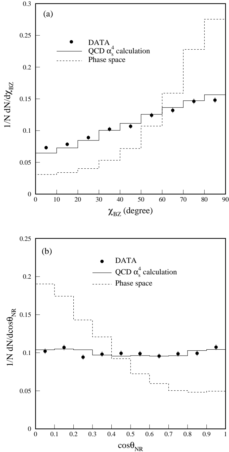
FIG. 11. The distribution of the angle between the planes of (a) the two leading jets and the two non-leading jets and (b) the momentum vector differences of the two leading jets and the two non-leading jets, for four-jet events in their center-of-mass system. Only statistical errors are shown. The RMS of the fractional differences is 5.7% for \chi_{BZ} and 4.1% for \cos\theta_{NR} . The estimated systematic uncertainty on the measurement is 6%. The data are also listed in Table VIII.
