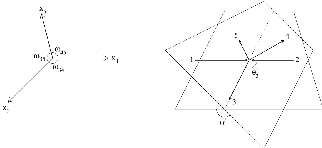
FIG. 1. Illustration of the topological variables: x_i , \omega_{ij} , \theta_3^* and \psi^* for the three-jet events.
