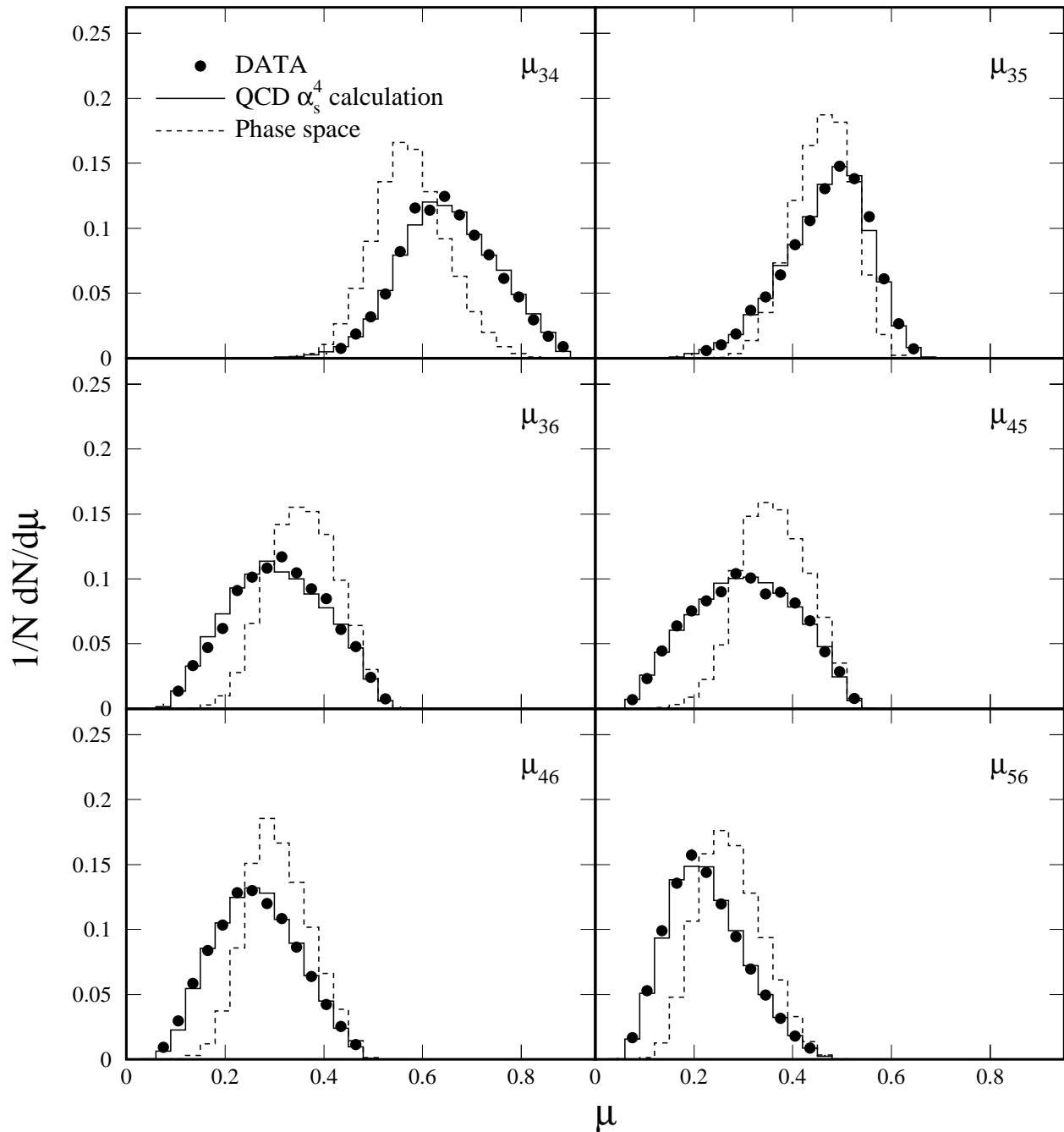
FIG. 10. Distributions of scaled jet pair mass for the four-jet events in their center-of-mass system. Only statistical errors are shown. The RMS's of the fractional differences between the data and QCD for the six masses are 7.8%, 7.1%, 6.8%, 6.3%, 4.1% and 3.7%. The estimated systematic uncertainty on the measurement is 6%. The data are also listed in Table VII.
